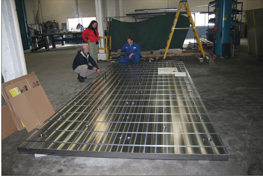
(left) Steel T-slot base plate 8' x 18' manufactured for Clemson University
